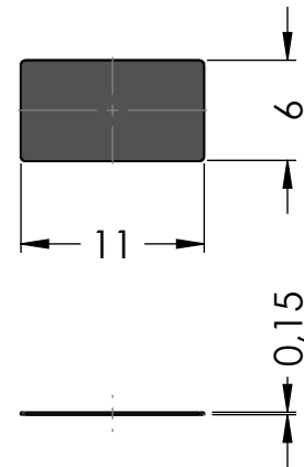
PART DETAIL
