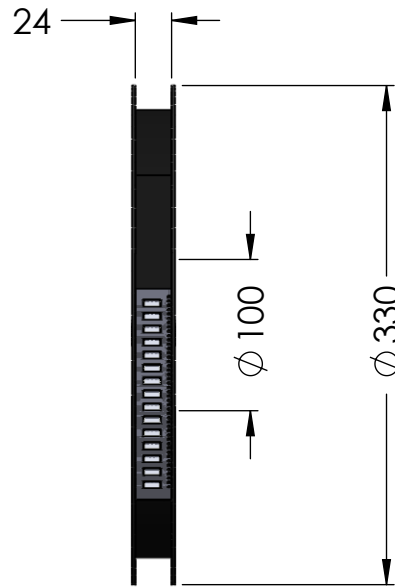
Reel detail
