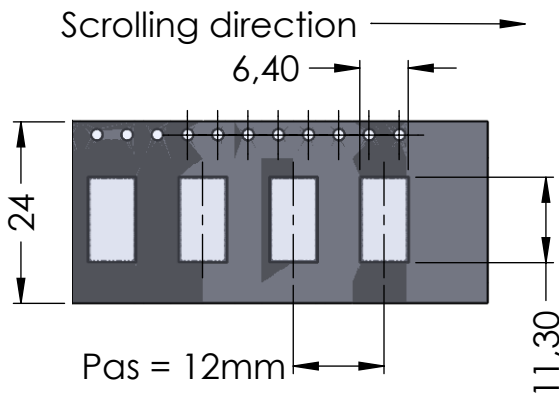
DETAIL VIEW OF CARRIER TAPE
