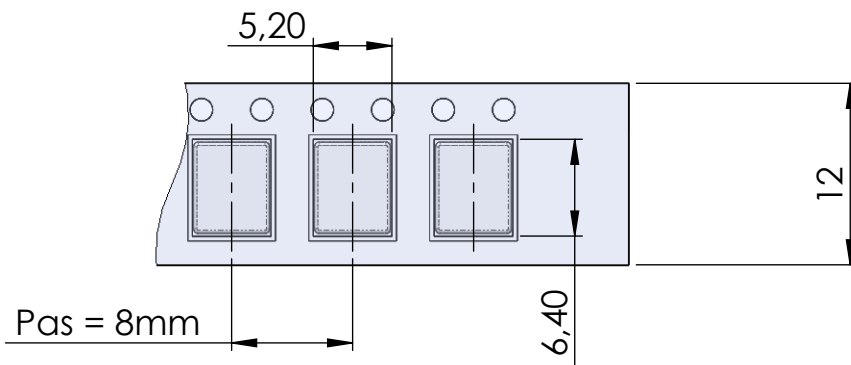
DETAIL VIEW OF CARRIER TAPE
